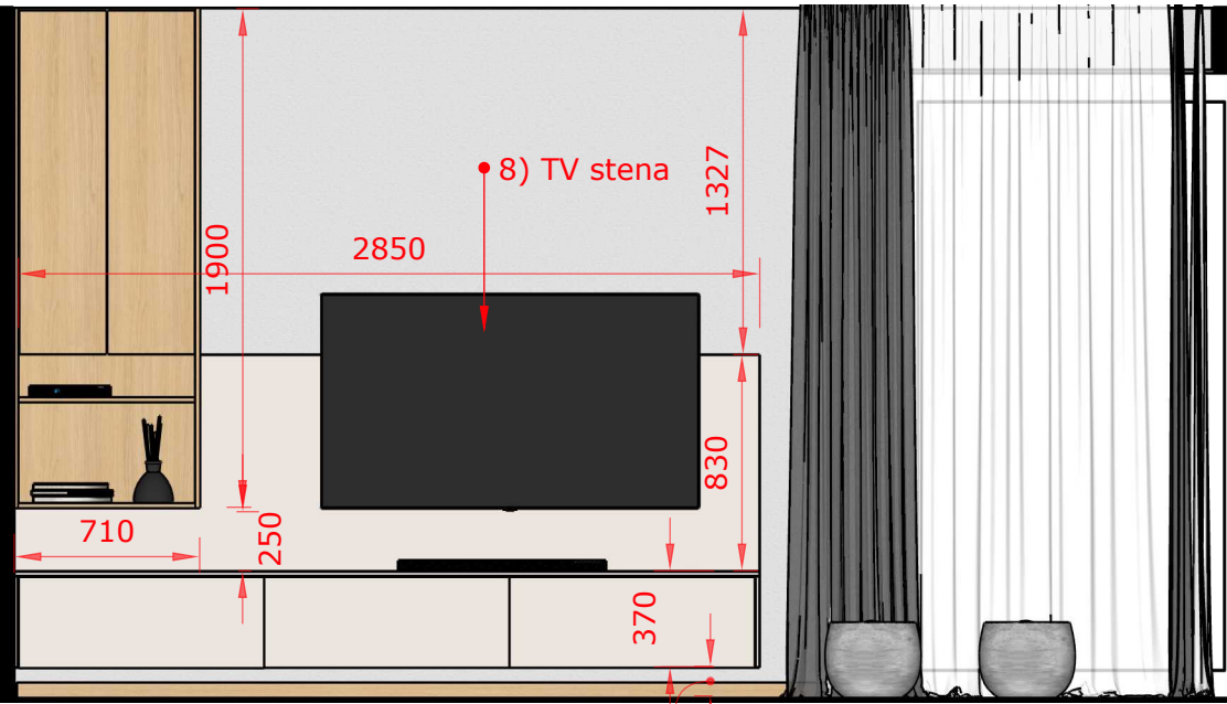
Rez 2
