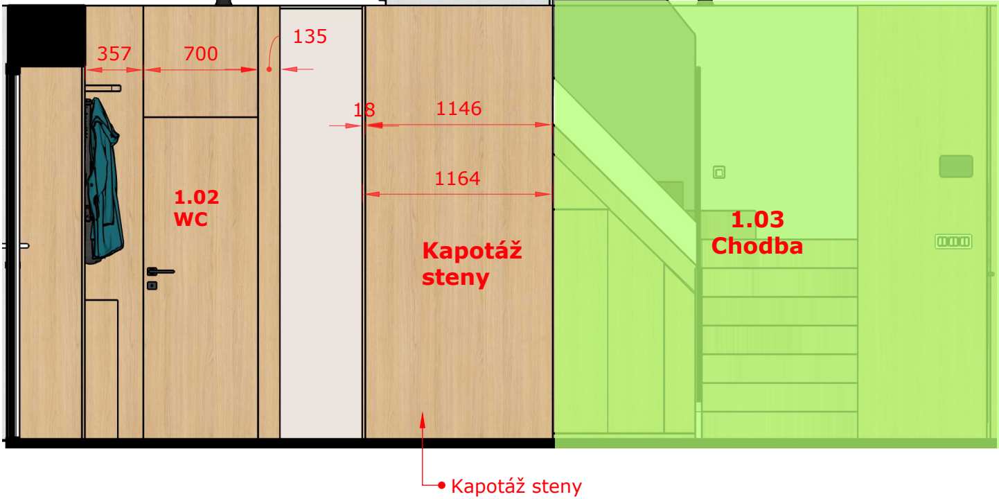
Rez 4
